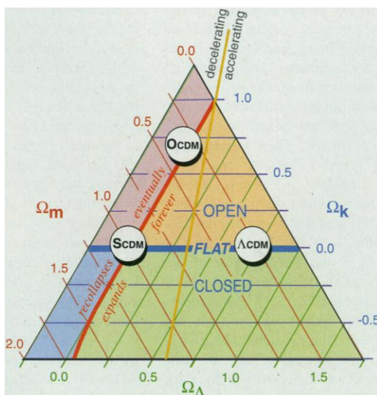
Fig. 1 (left). The Cosmic Triangle.
